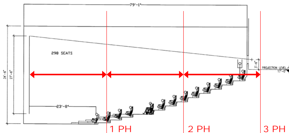
Architectural elevation of a modern 298-seat "stadium seating" auditorium. We have marked viewing distances in Picture Heights (PH). The first row is less than one PH from the screen.
